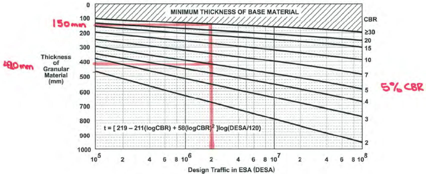
Figure 8.4: Design chart for granular pavements with thin bituminous surfacing
