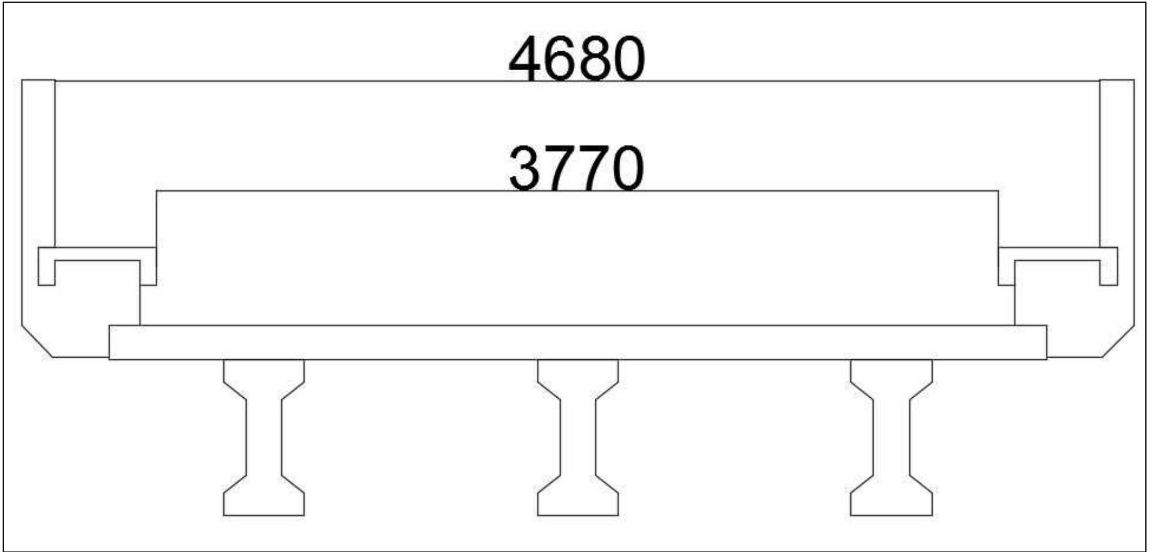
Existing structure
