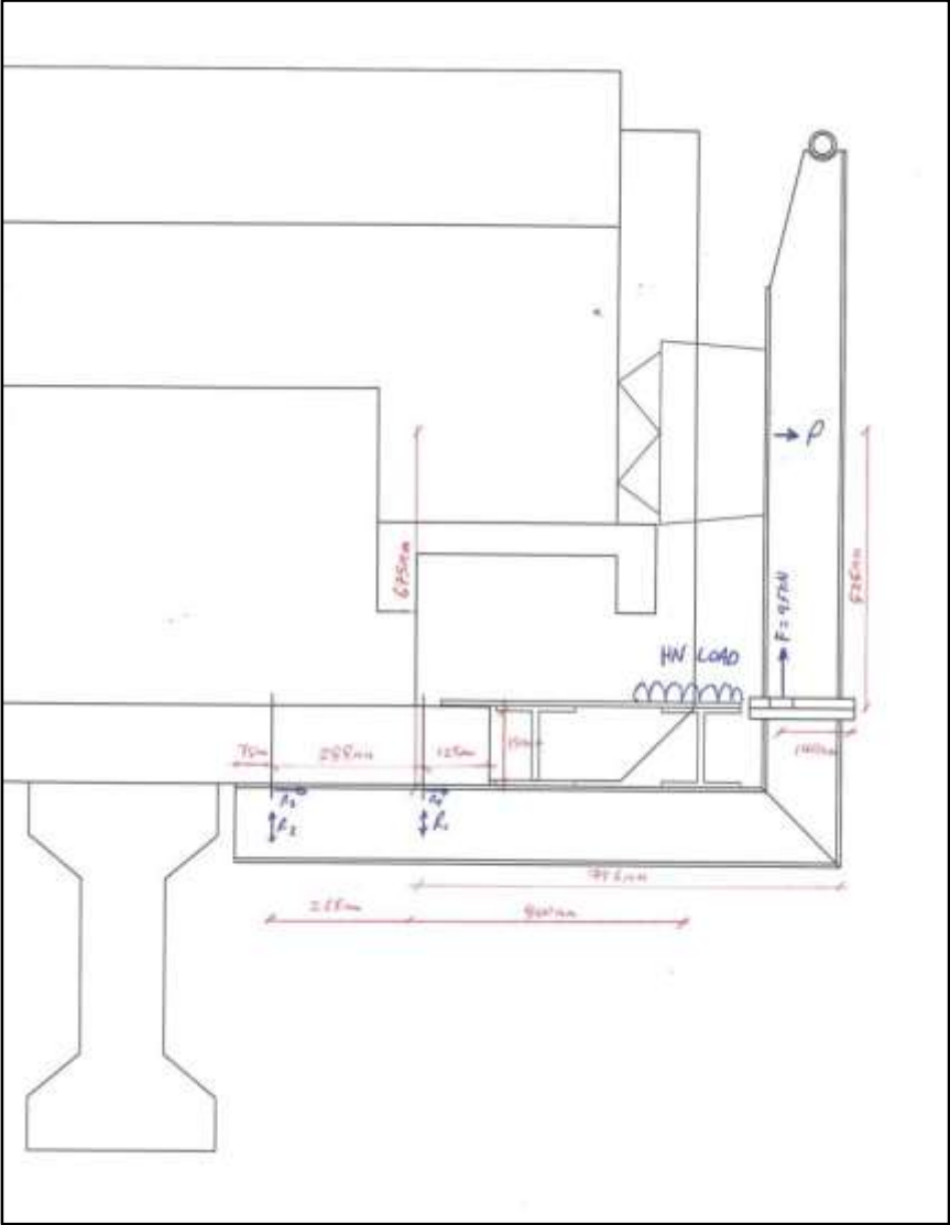
Loading diagram
